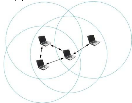
Figure 3: AdHoc Network
